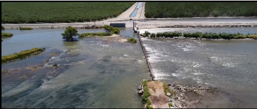
Kings River flood releases from Pine Flat Dam flowing west through the James Weir are diverted into the District's Main Canal for irrigation & recharge. Excess flows continue west toward Tranquillity Irrigation District & into the Mendota Pool. - June, 2023
